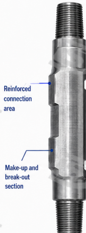
TOOL JOINT
